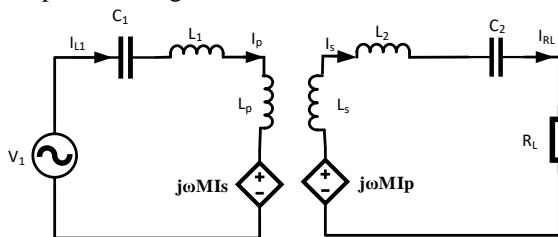
Fig. 3. Equivalent analytical circuit of the LCLCL-T topology.
